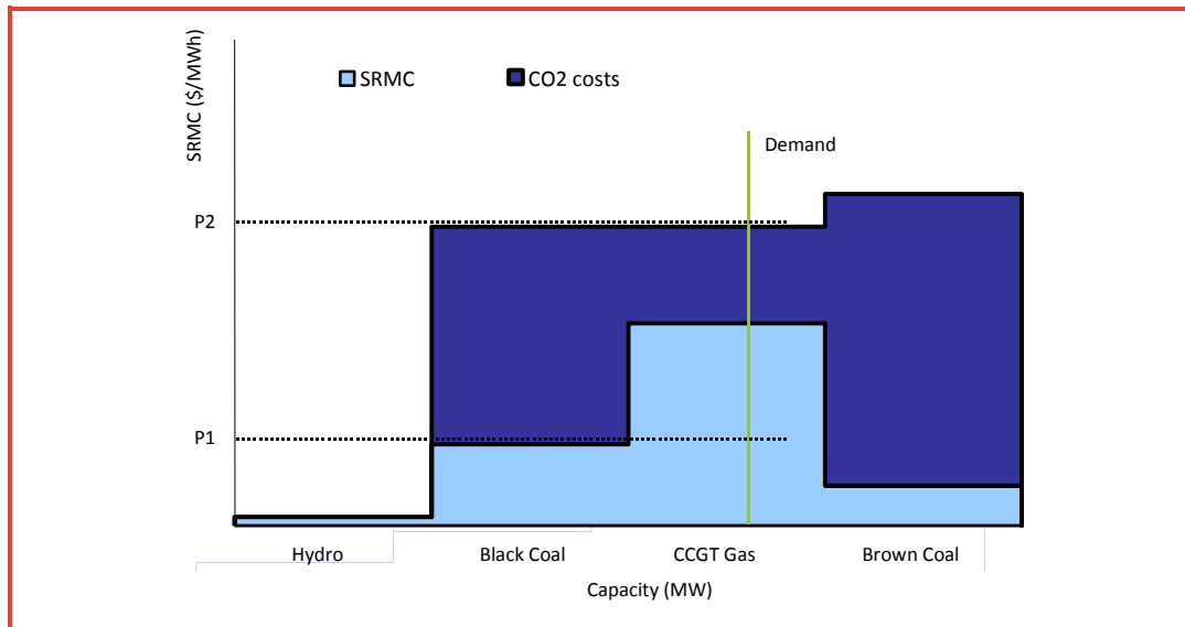
Figure 7: Stylised example of carbon costs: with change in merit order
