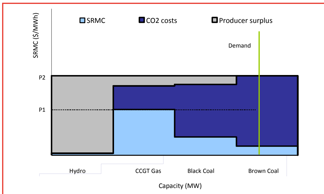
Figure 10: Merit order with an ETS (High carbon price)
