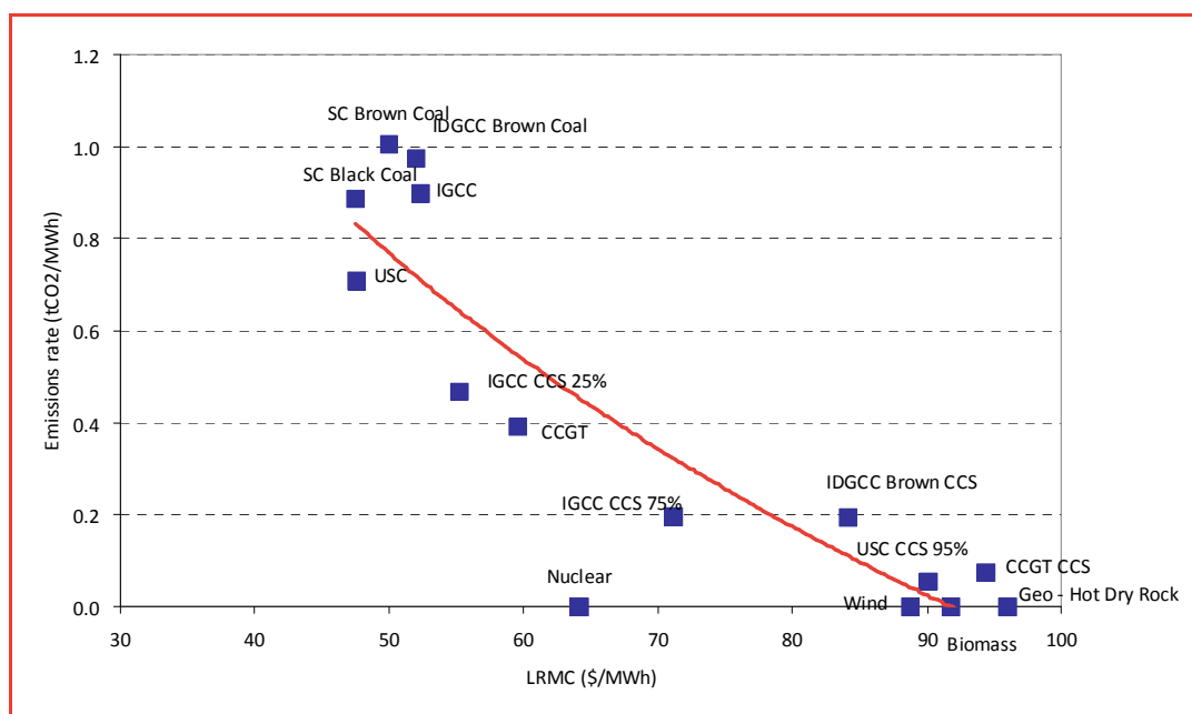
Figure 15: LRMC and emissions intensity trade-off
