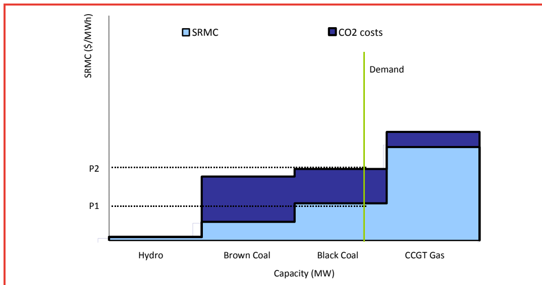
Figure 6: Stylised example of carbon costs: no change in merit order
