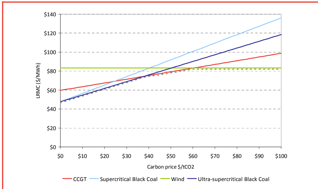
Figure 16: Carbon prices and generation costs
