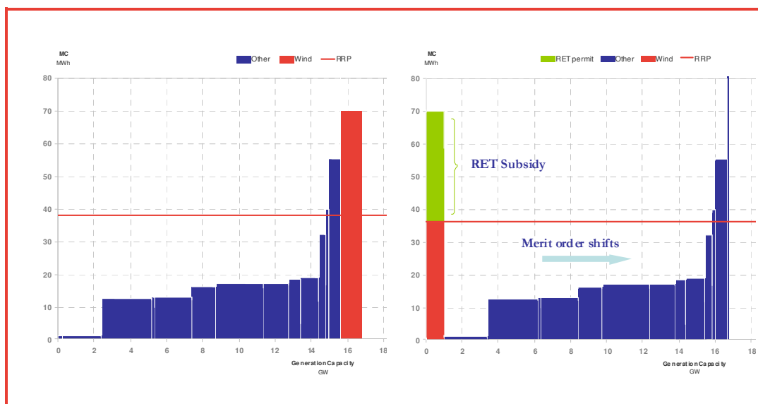
Figure 19: Impact of a renewable energy target on the merit order
