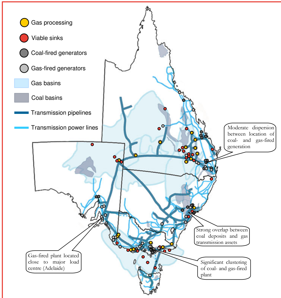
Figure 17: The NEM's key gas and electricity infrastructure
