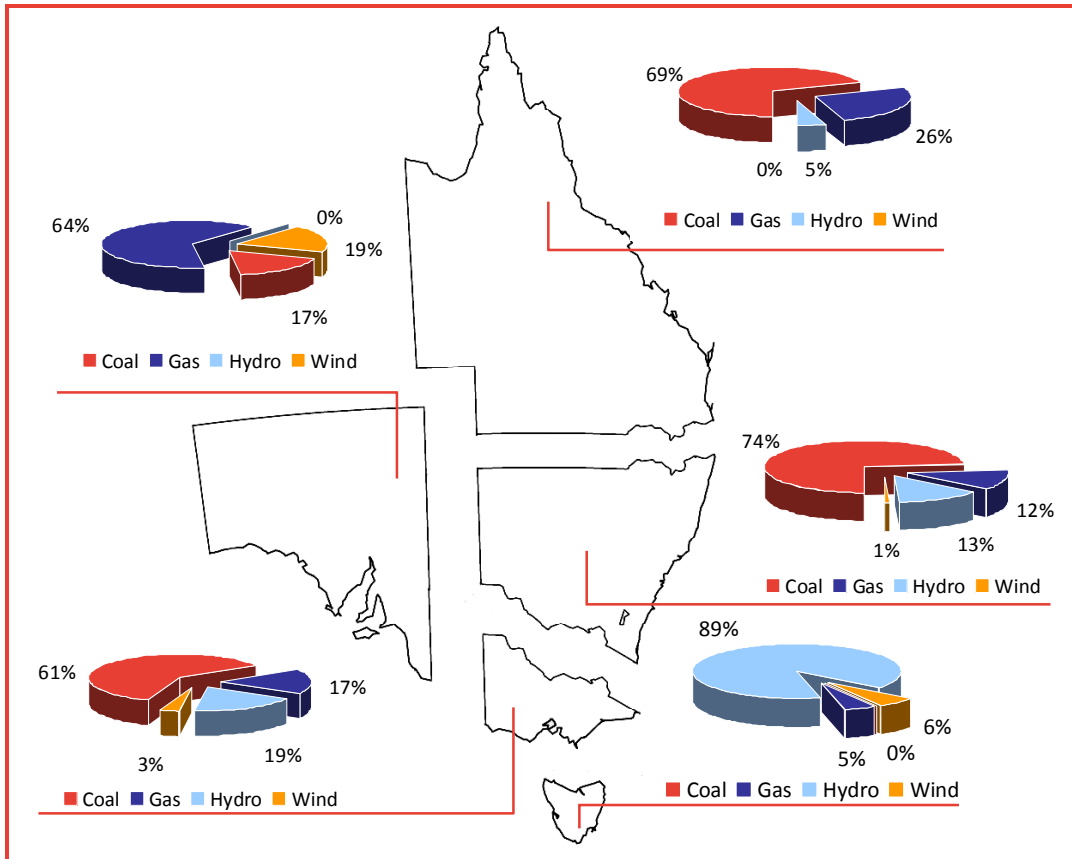
Figure 5: Expected 2010 installed capacity by region and technology
