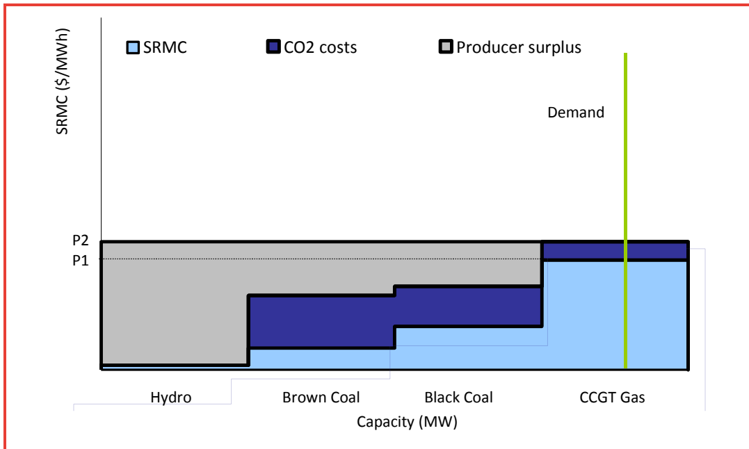
Figure 9 Merit order with an ETS (Low carbon price)
