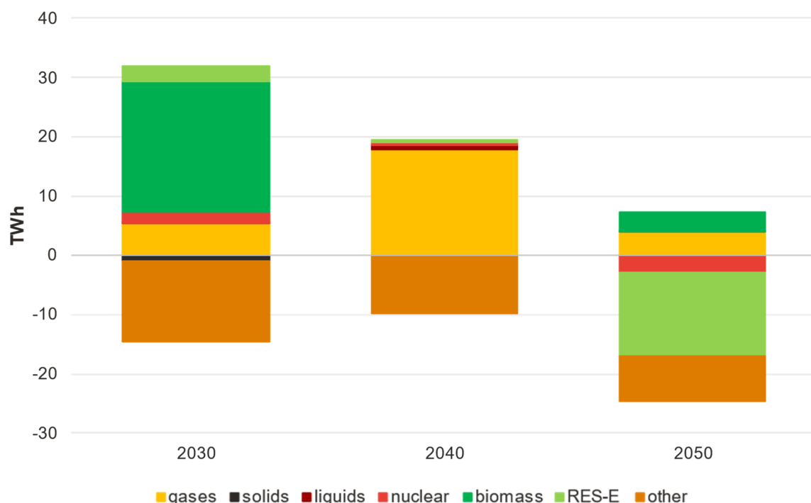
Figure 39 Difference in primary energy supply (EU27, What-if Delayed Grid)
